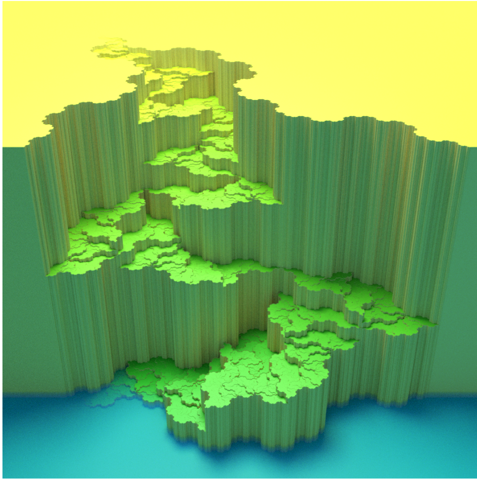
Figure 5: The BMTV triangle-filling curve visualised as an descending path by pftrail [4].
