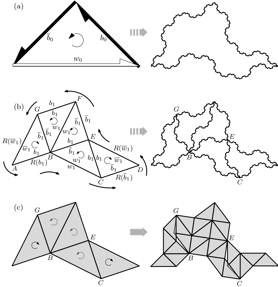
Figure 3: (a) The shape of the tiles. (b) Top-level tessellation and skeleton of the plane-filling curve. (c) In recursion, the approximating triangles do not tile the plane.
